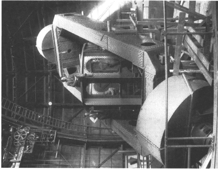
The 100-inch Telescope Under Construction
