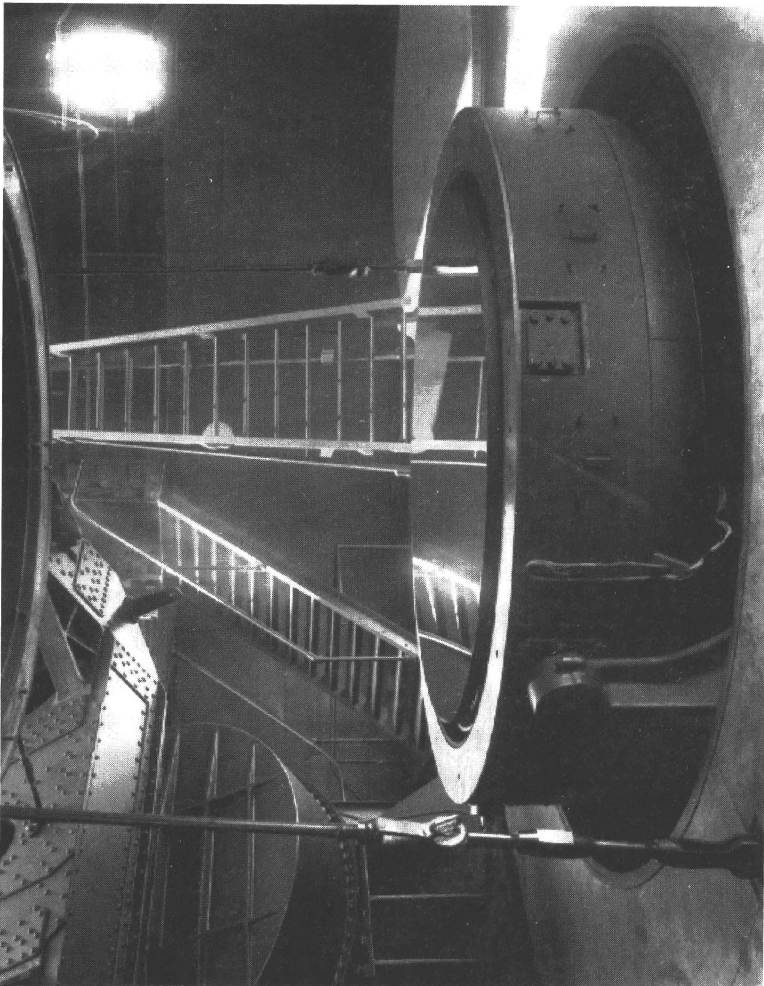
The 100-inch Mirror of the Hooker Telescope
