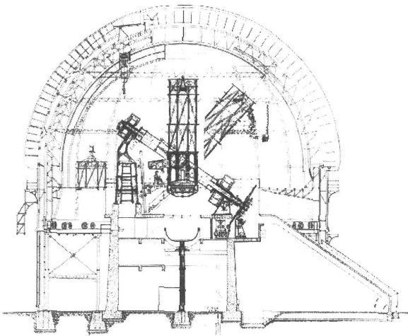
Diagrammatic drawing of the 100-inch Telescope
