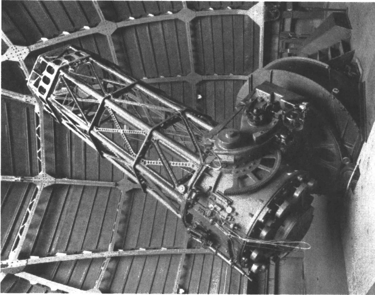
The 60-inch Reflector
